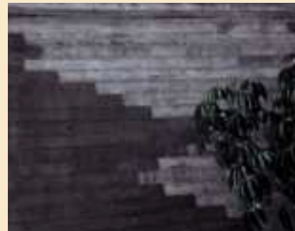
19. Variations in the porosity of lumber form work cause uneven absorption of water from the concrete, resulting in uneven color.
