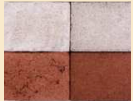
12. different water/cement ratios make plain (top) and colored concrete (bottom) appear pale or faded.
